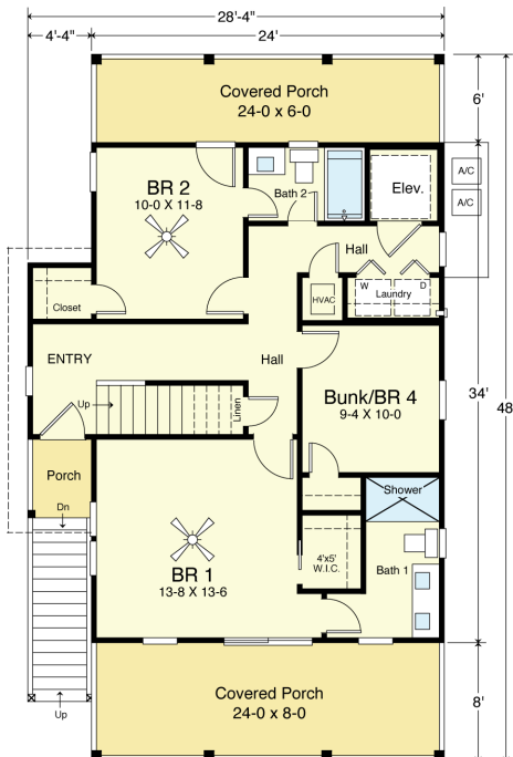
FIRST FLOOR PLAN 844.0 SF 9'-1 1/2" Ceilings
