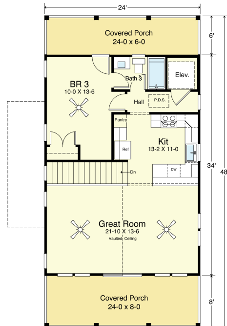
SECOND FLOOR PLAN 792.0 S.F. 9'-1 1/2" Ceilings
