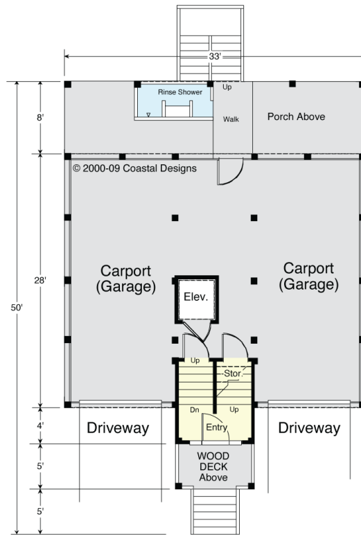
GROUND FLOOR PLAN 958.7 S.F. (Unheated)
