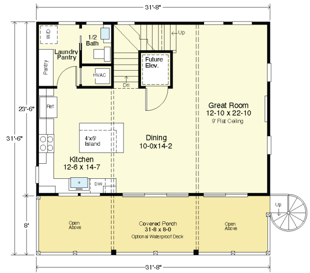
SECOND FLOOR PLAN 744.2 s.f. 9'-1 1/2" Flat Ceilings
