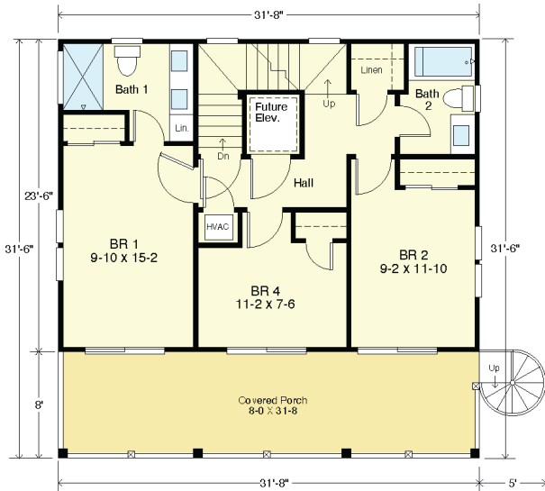
FIRST FLOOR PLAN 744.2 s.f. 8'-1 1/2" Flat Ceilings
