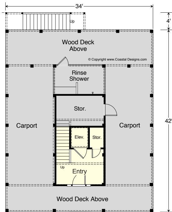
Ground Floor 240.0 s.f. (unheated)
