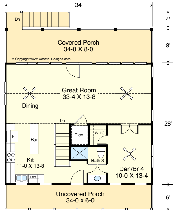
2nd Floor 952.0 sf
